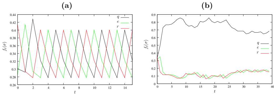
Figure 1. Examples of evolutions observed on the fractions f_t(\sigma) with \sigma \in S = \{q, e, r\} ( i.e. at the macroscopic level) for \lambda -Poisson networks with typical (0.3, 0.3, 0.4) -initial states. (a) for a (typical) 10-Poisson network. (b) for a (non-typical) 1-Poisson network.
